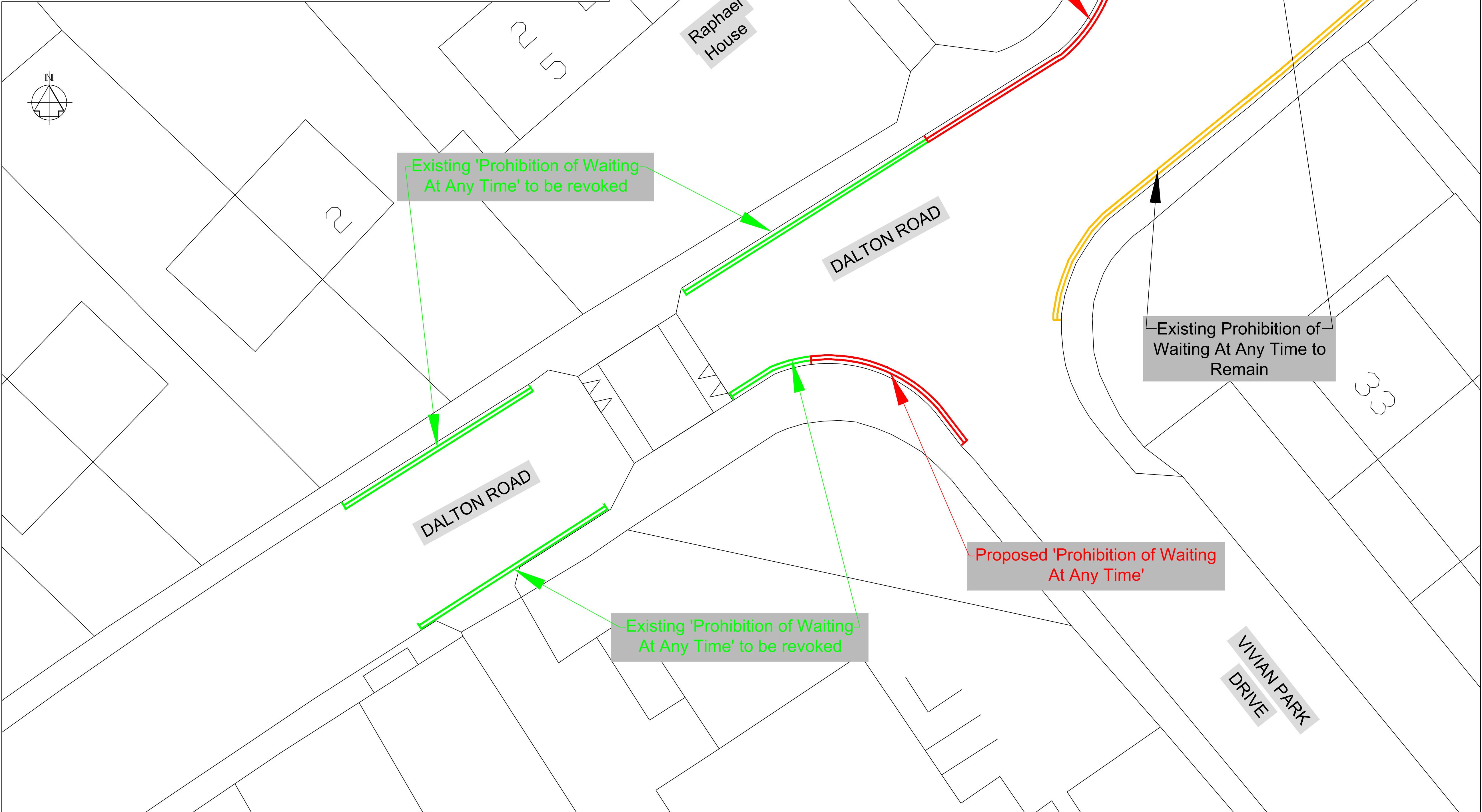
DALTON ROAD PROPOSED TRAFFIC REGULATION ORDER LAYOUT - NOT TO SCALE
